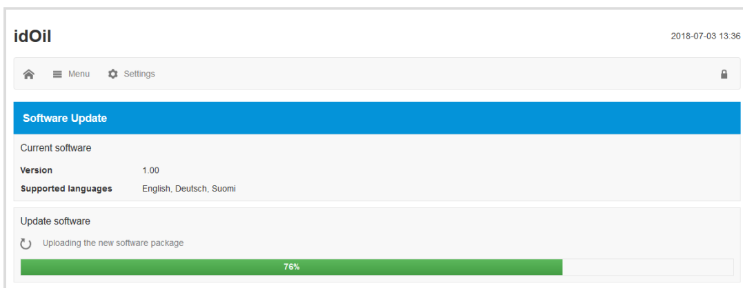
Figur 42. Softwareupload
