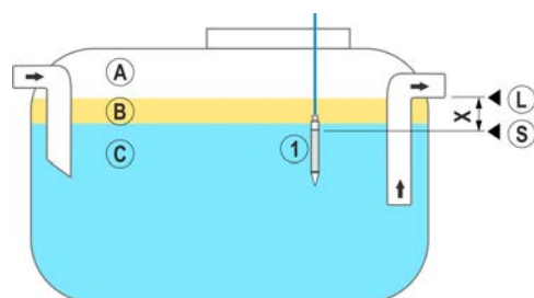
Figur 10. Installation af idOil-OIL-sensoren
